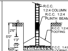
FOUNDATION DETAIL
