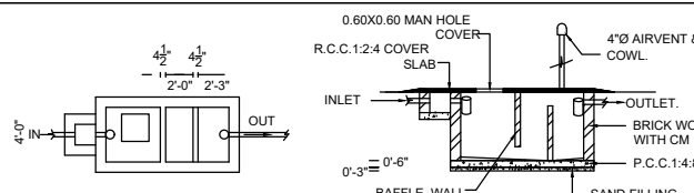
SEPTIC TANK DETAIL
