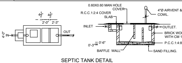
SEPTIC TANK DETAIL
