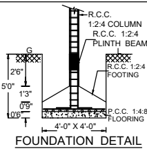
FOUNDATION DETAIL
