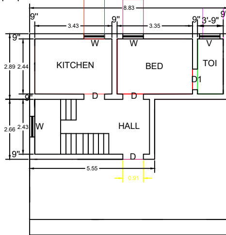
PROPOSED F.F. PLAN
