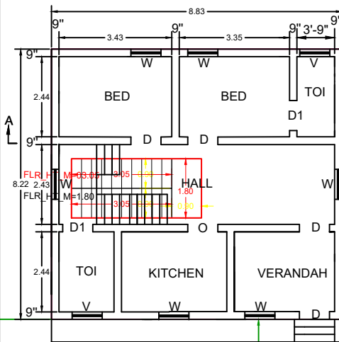
EXISTING+PROPOSED G.F. PLAN
