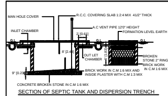
SECTION OF SEPTIC TANK AND DISPERSION TRENCH
