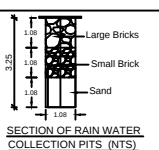
SECTION OF RAIN WATER COLLECTION PITS (NTS)
