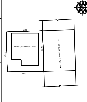
SITE PLAN
