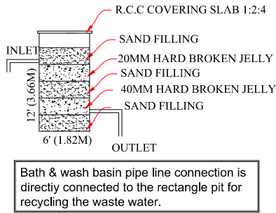
Waste Water Recycle Unit Not To Scale
