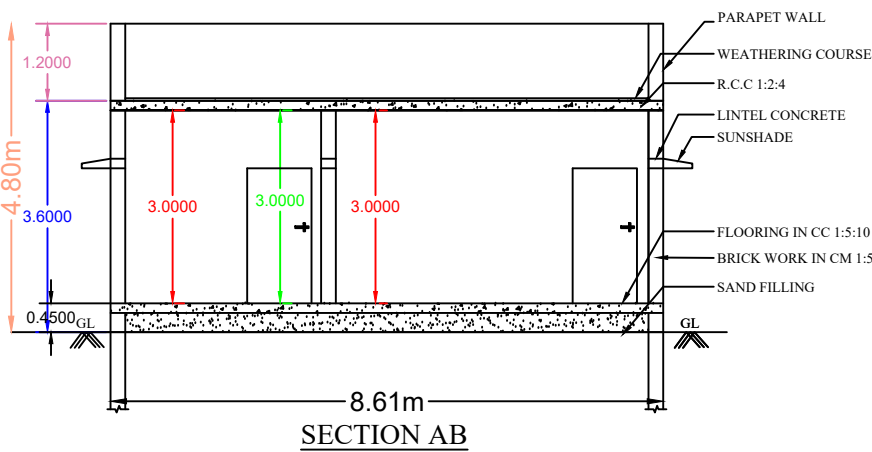
SECTION AB
