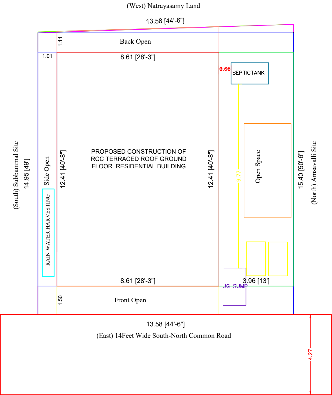
SITE PLAN
