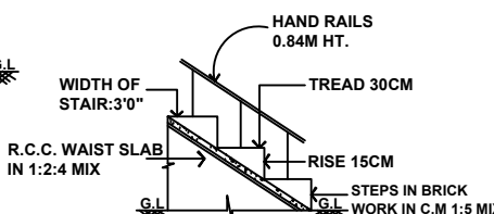
STAIR CASE DETAILS (NOT TO SCALE)
