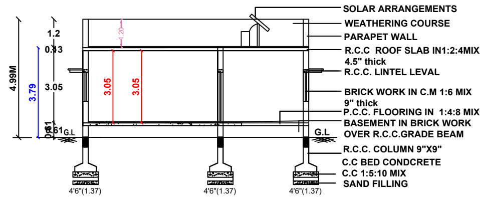
SECTION " AB "
