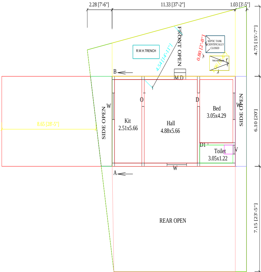
ALTERATION ON FIRST FLOOR (Shop To Residential in FF)
