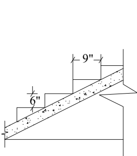
Staircase Detail Not To Scale
