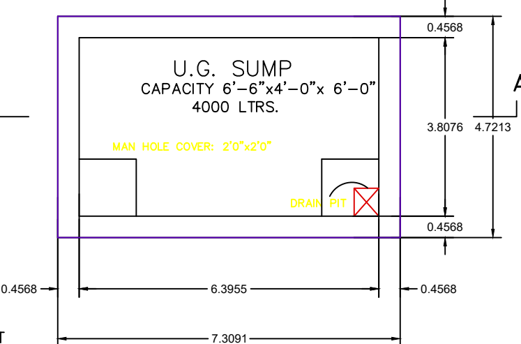
SUMP DETAIL SCALE 1"=4'0"
