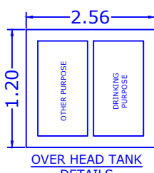
OVER HEAD TANK DETAILS
