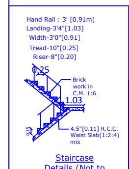
Staircase Details (Not to scale)
