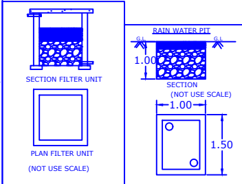
PLAN OF RAIN WATER HARVESTING
