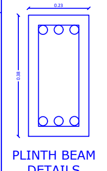
PLINTH BEAM DETAILS
