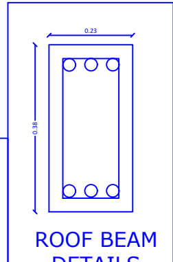
ROOF BEAM DETAILS
