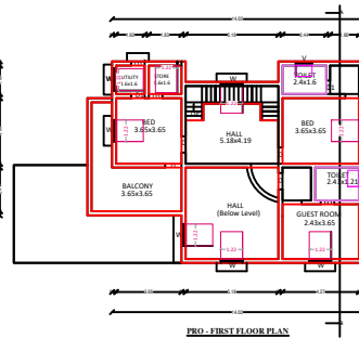
PRO - FIRST FLOOR PLAN
