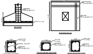
DETAILS OF THE PROPOSED BUILDING (NTS)
