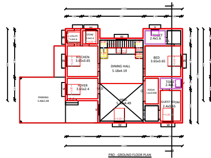
PRO - GROUND FLOOR PLAN
