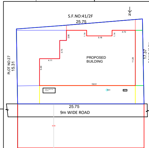
DETAILS OF THE PROPOSED BUILDING (NTS)
