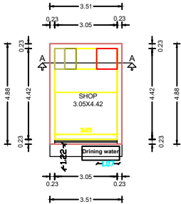
GROUND FLOOR PLAN COMMERCIAL
