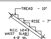
STAIRCASE DETAILS (NTS)
