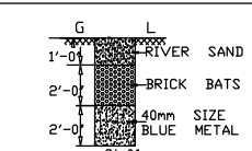
RAIN WATER PERCOLATION PIT ( NTS )
