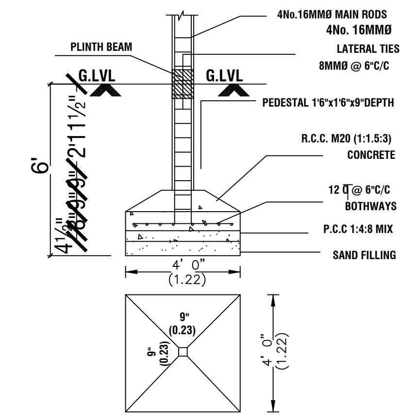
FOUNDATION DETAIL
