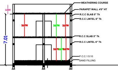
Section - AA Section
