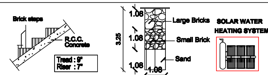
STAIRCASE DETAILS
