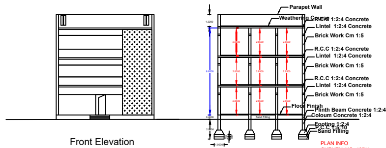
Section Section AA
