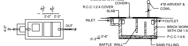
SEPTIC TANK DETAIL
