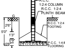
FOUNDATION DETAIL
