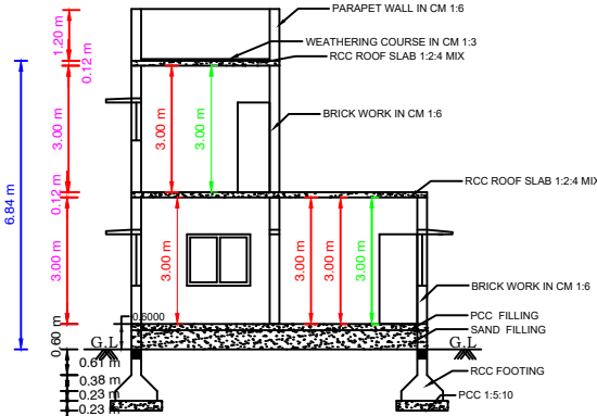
SECTION OF KA
