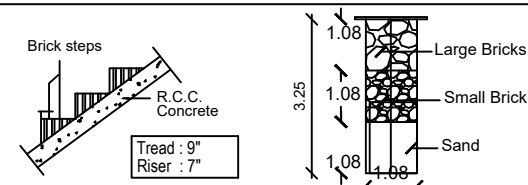
STAIRCASE DETAILS
