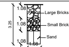
SECTION OF RAIN WATER
