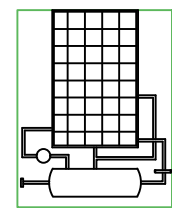
SOLAR SYSTEM
