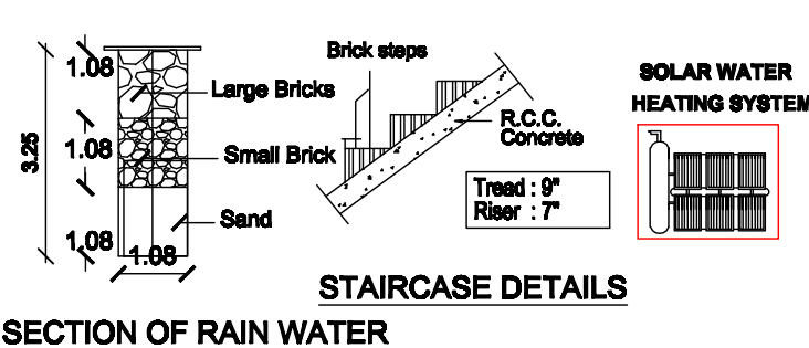
SECTION OF RAIN WATER
