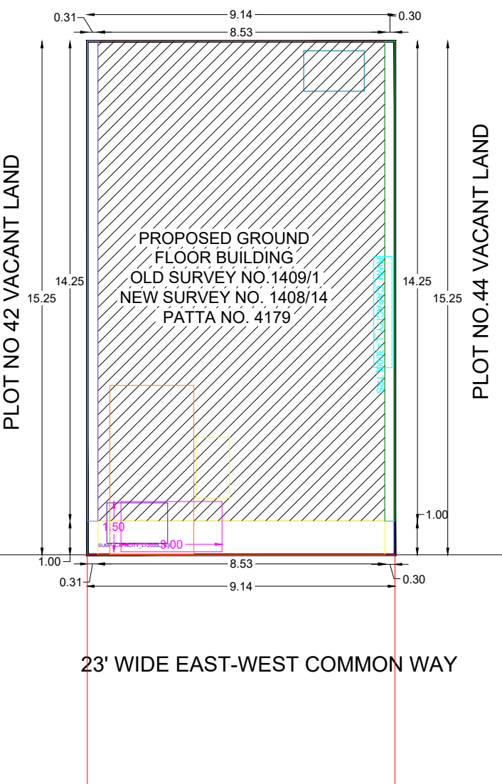
SITE PLAN
