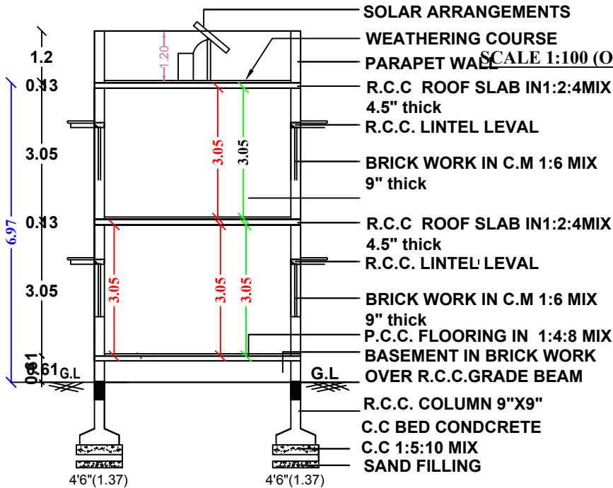
SECTION " AB "
