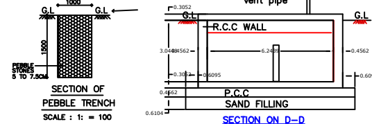
SECTION OF PEBBLE TRENCH
