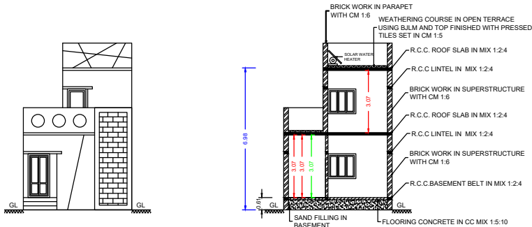
FRONT ELEVATION
