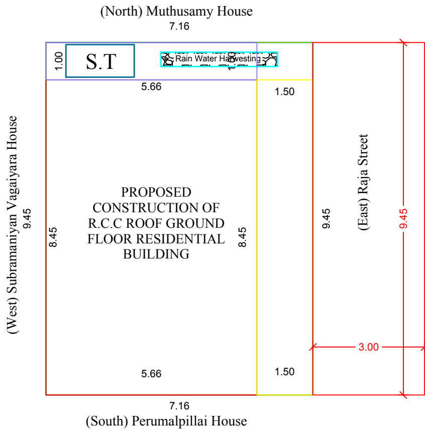
SITE PLAN
