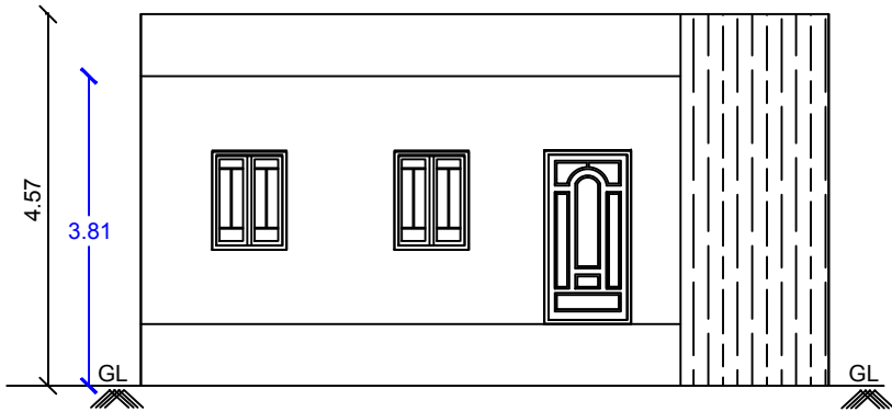
FRONT ELEVATION (EAST FACING)
