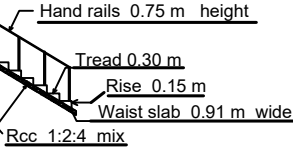
Staircase Details
