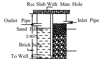
RWH TANK DETAILS
