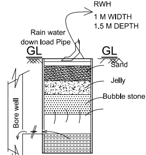
SEC. RAIN WATER HARVEST PIT
