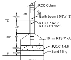
FOUNDATION DETAILS
