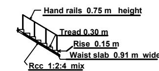
Staircase Details
