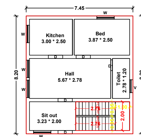
APPROVED GROUND FLOOR PLAN
