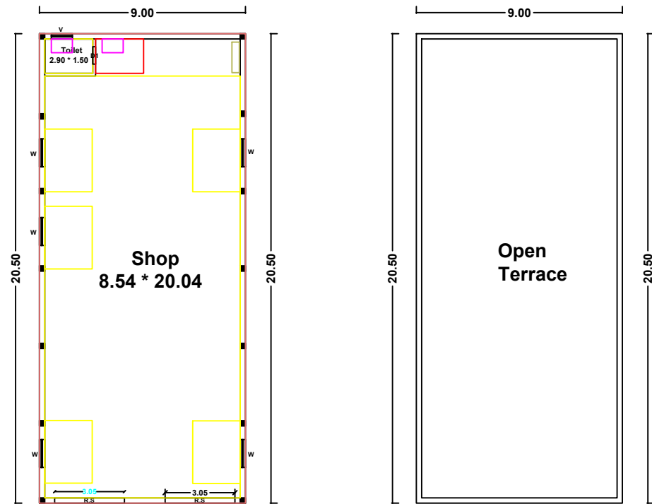
PROPOSED GROUND FLOOR - SHOP BUILDING
