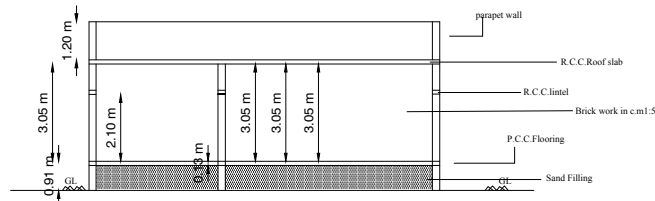
SECTION-SR
