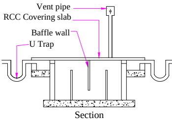
SECTION - 'CD'
