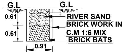
. SECTION ON RAIN WATER COLLECTION TUB .
