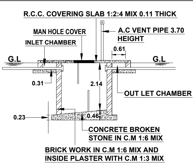
.SECTION ON SEPTIC TANK .
