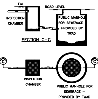
WASTE DISPOSAL DETAIL
