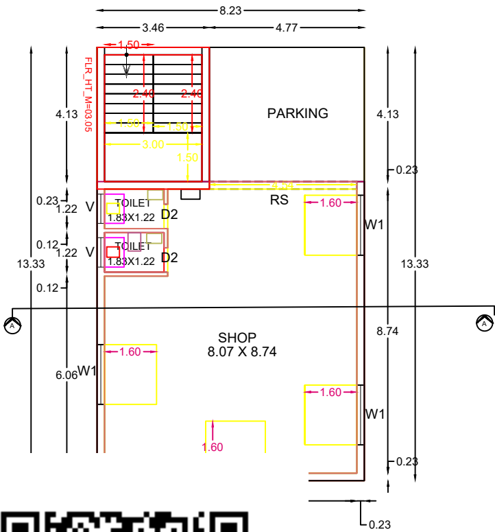
FLOOR PLAN
