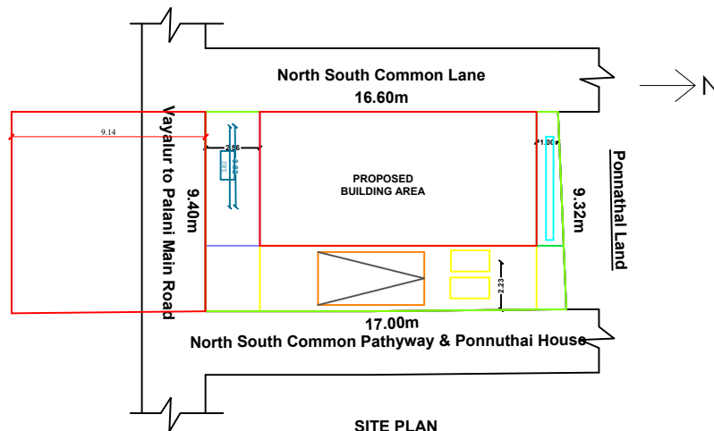
SITE PLAN
