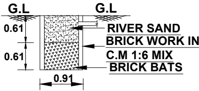
. SECTION ON RAIN WATER COLLECTION TUB .
