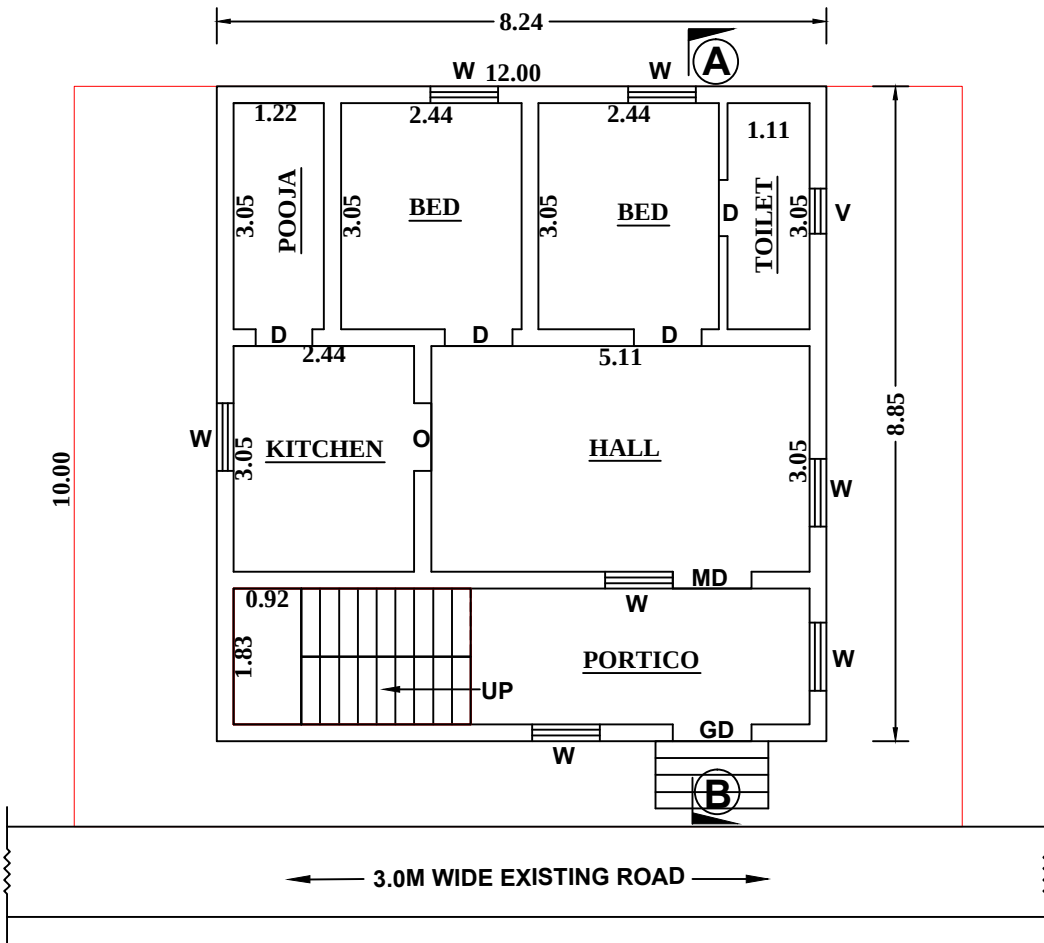
. GROUND PLAN .
