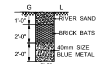
RAIN WATER PERCOLATION PIT (NTS)
