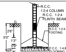
FOUNDATION DETAIL
