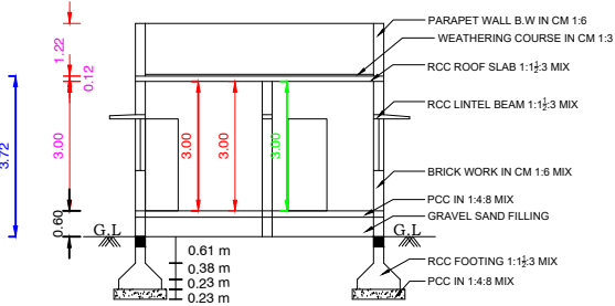
SECTION ON KA
