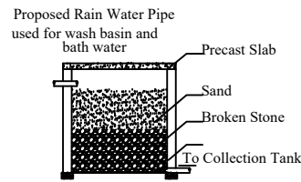
Section of Filter Unit
