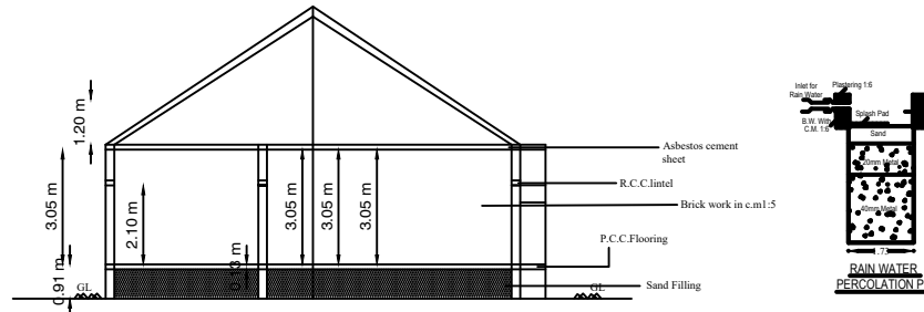
SECTION-AB
