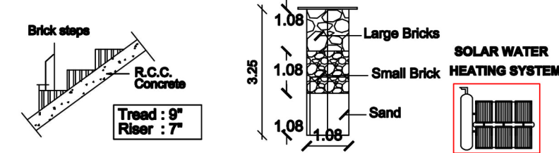
STAIRCASE DETAILS
