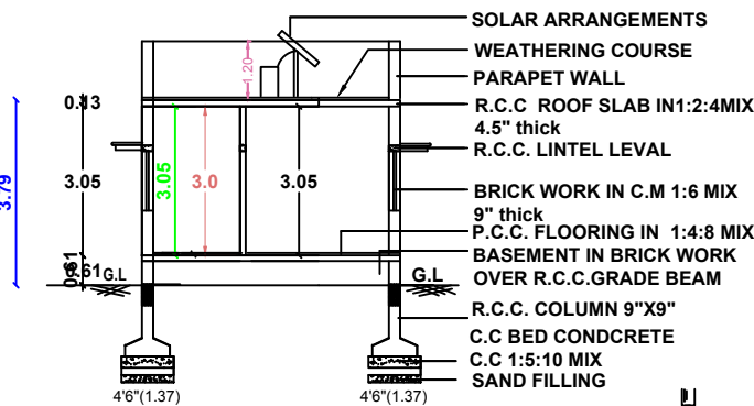
SECTION " AB "
