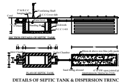
DETAILS OF SEPTIC TANK & DISPERSION TRENCH
