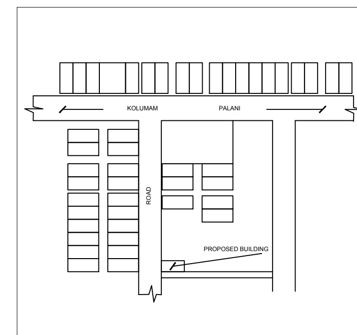
TOPO PLAN
