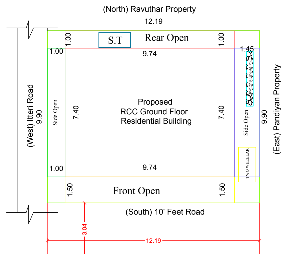
SITE PLAN
