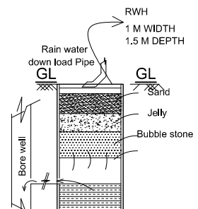
SEC. RAIN WATER HARVEST PIT
