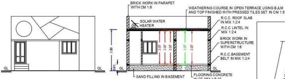
FRONT ELEVATION
