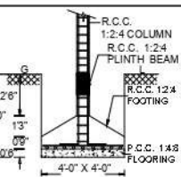
FOUNDATION DETAIL
