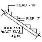
STAIRCASE DETAILS (NTS)
