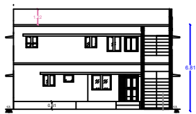
ELEVATION FACING EAST
