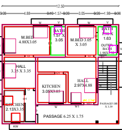
FIRST FLOOR FACING EAST
