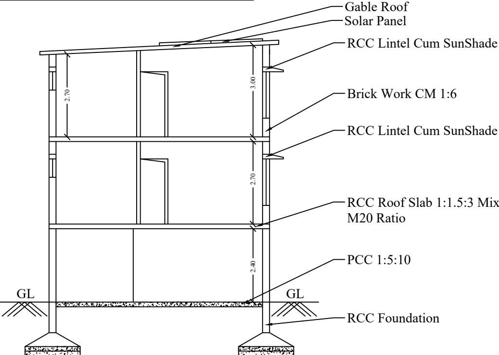
Cross Section on 'AB'
