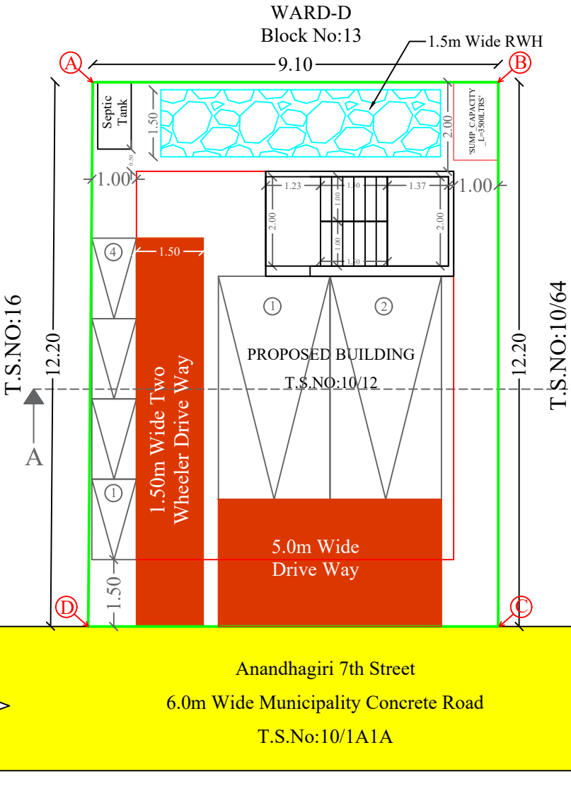
Site Cum Stilt Floor Plan
