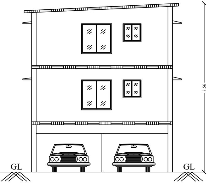
Front Elevation
