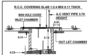
.SECTION ON SEPTIC TANK .
