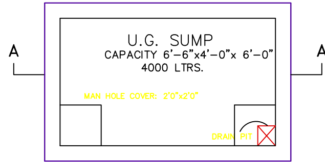
SUMP DETAIL SCALE 1"=4'0"
