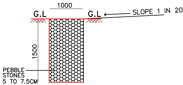
SECTION OF PEBBLE TRENCH SCALE : 1: = 100
