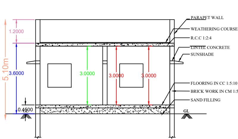
SECTION AB
